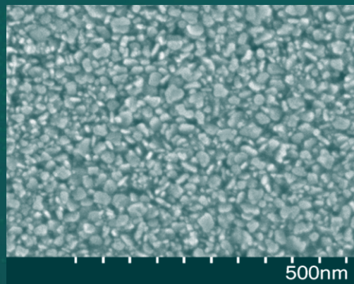
BaFe Particle
