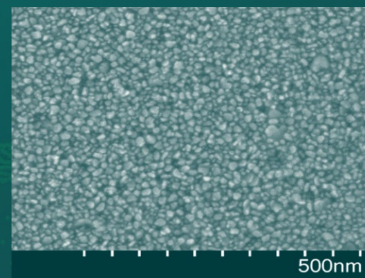
SrFe Particle
